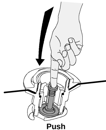
Deflation position
