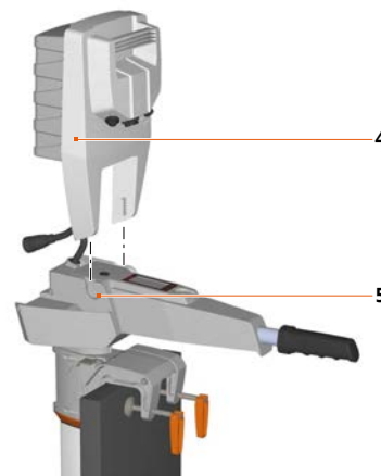
Fig. 44: Battery installation
