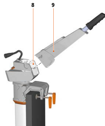
Fig. 65: Removing the tiller
