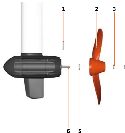
Fig. 67: Travel 1103 propeller attachment
