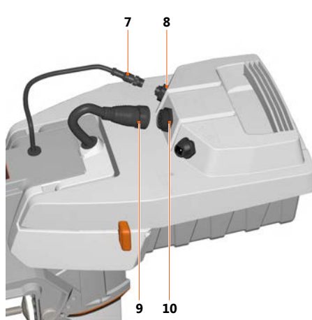
Fig. 46: Electrical connections
