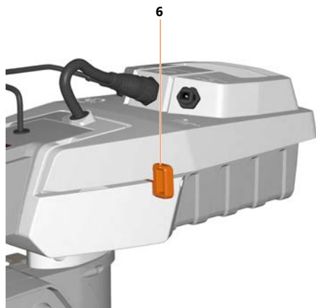
Fig. 45: Locking pin
