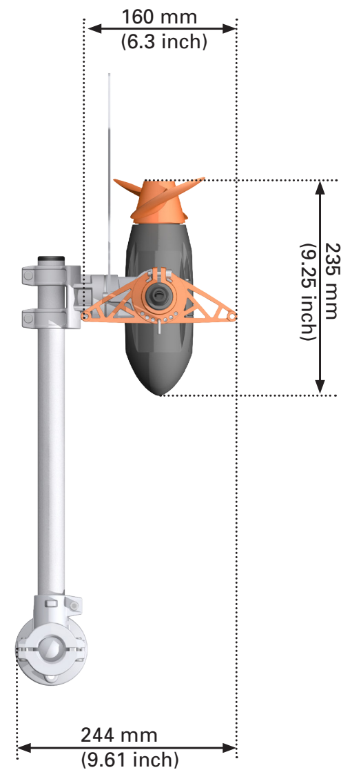
Torqeedo Ultralight 403
