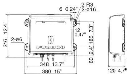
Network Multibeam Sonar DFF3D
