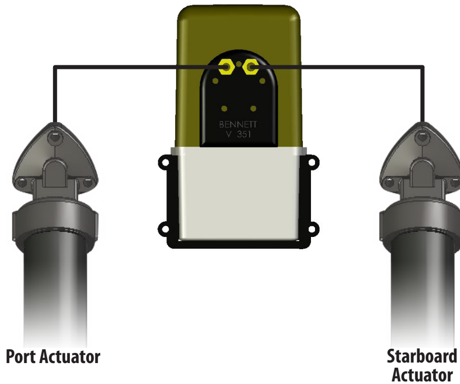
Tubing Diagram for Single Actuator System
