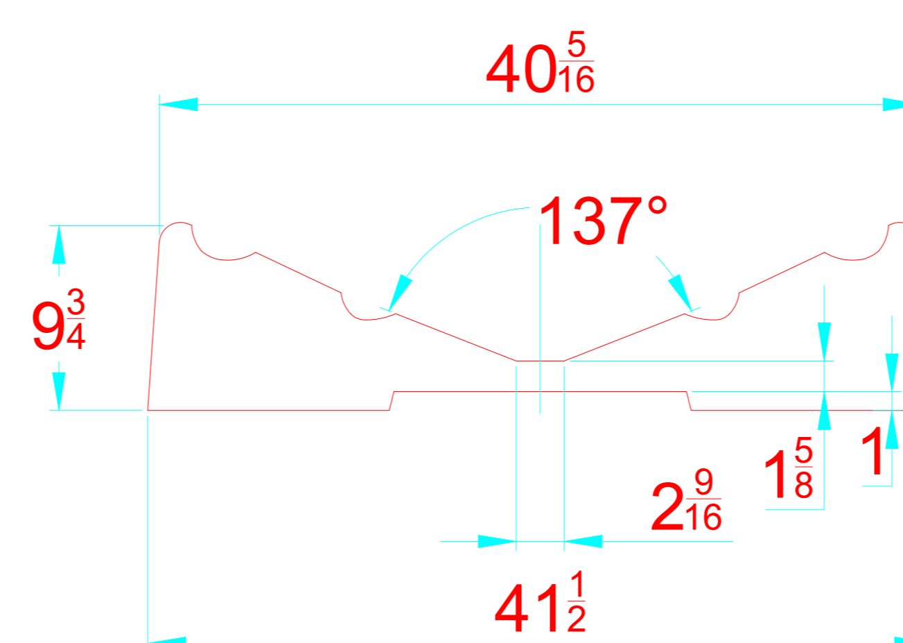
TRANSVERSAL SECTION "A" SECCION TRANSVERSAL "A"
