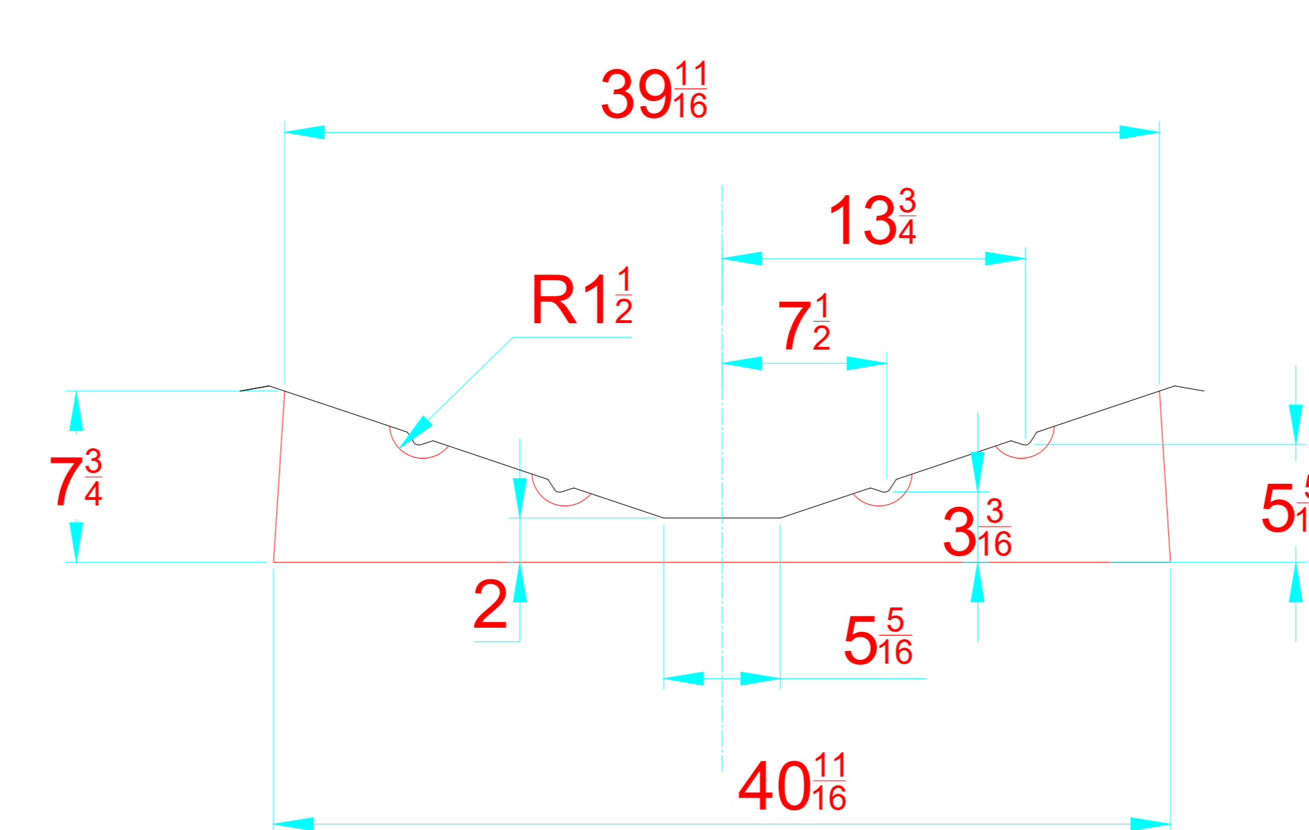
TRANSVERSAL SECTION "A" SECCION TRANSVERSAL "A"
