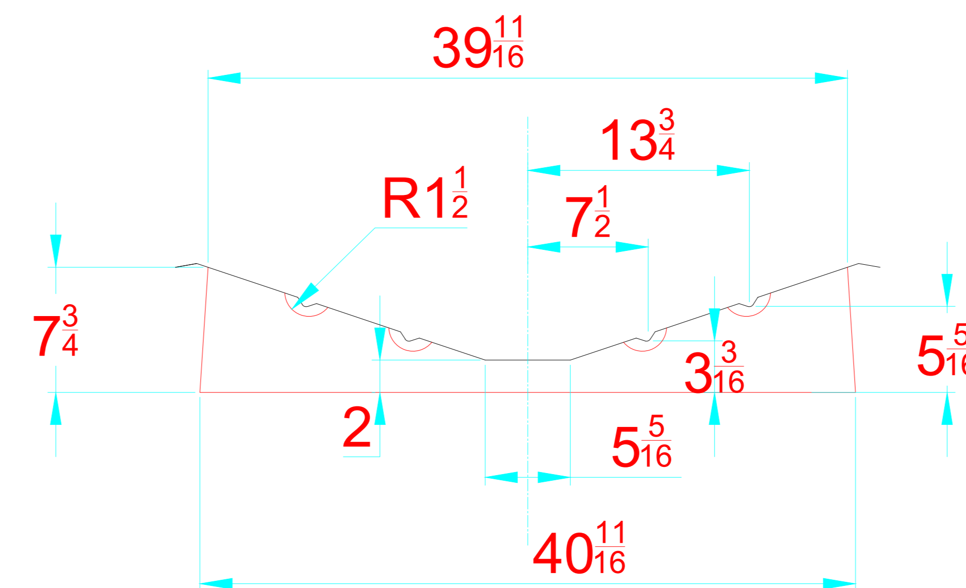
TRANSVERSAL SECTION "A" SECCION TRANSVERSAL "A"
