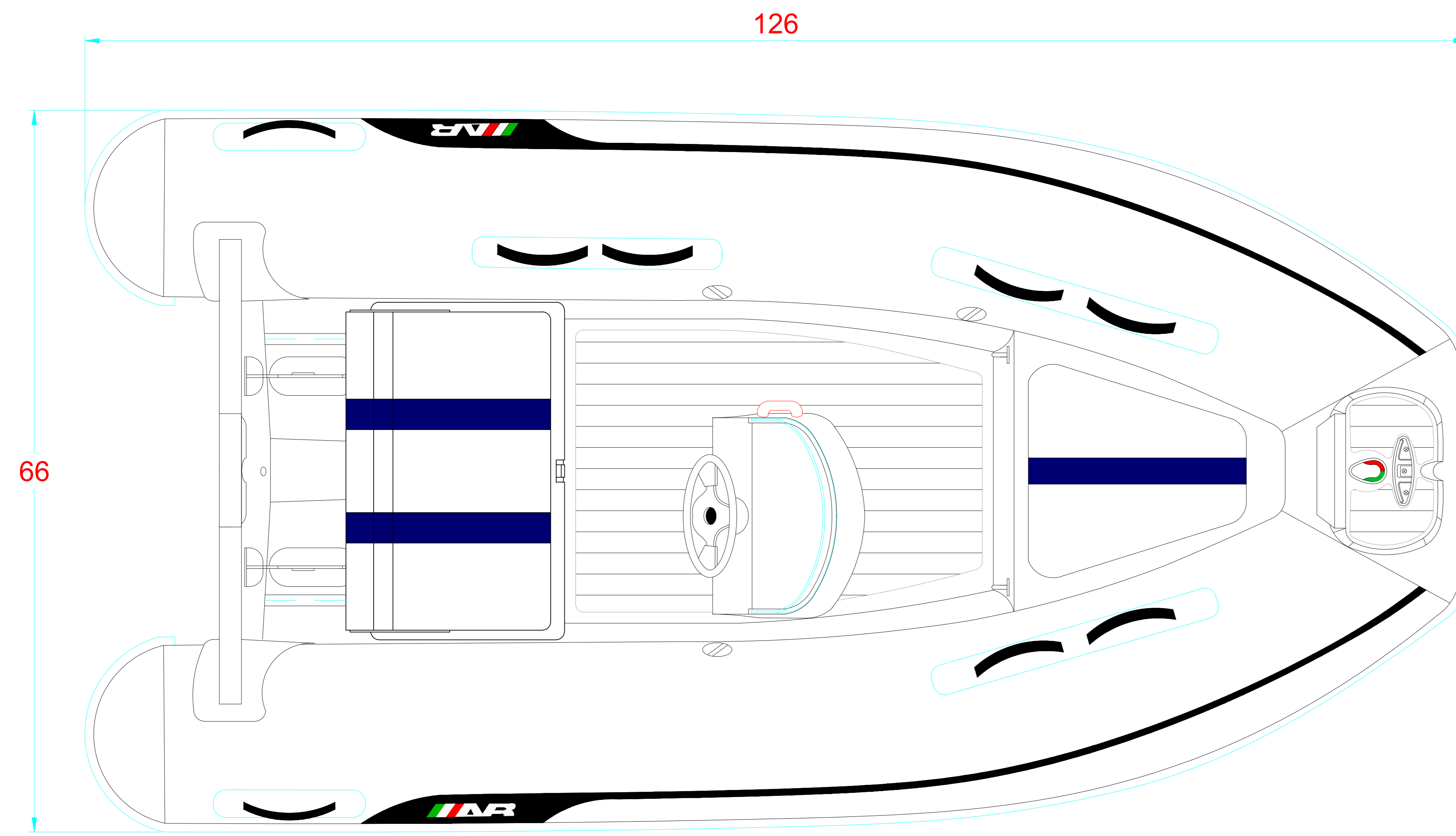
PLANT VIEW VISTA SUPERIOR
