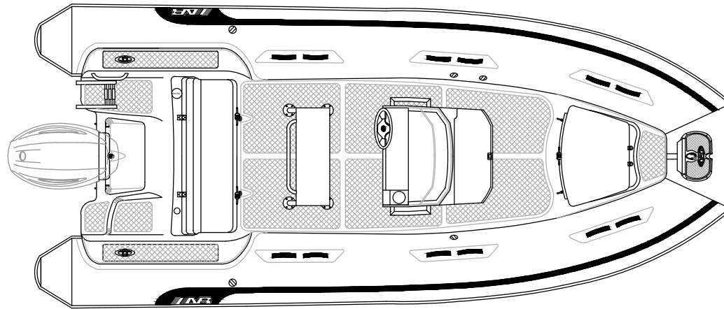
PLANT VIEW
